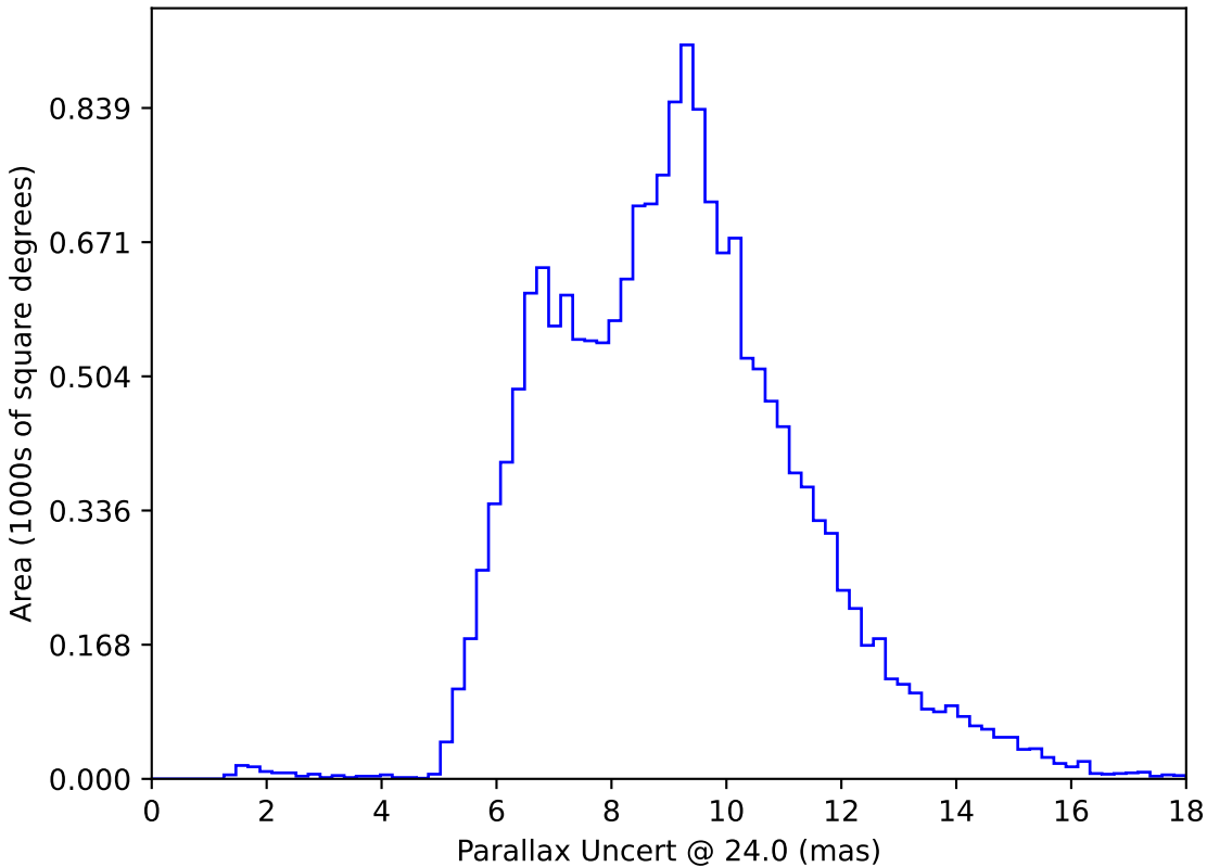
weather_cloudso36v3.4_10yrs WFD: Parallax Uncert @ 24.0
