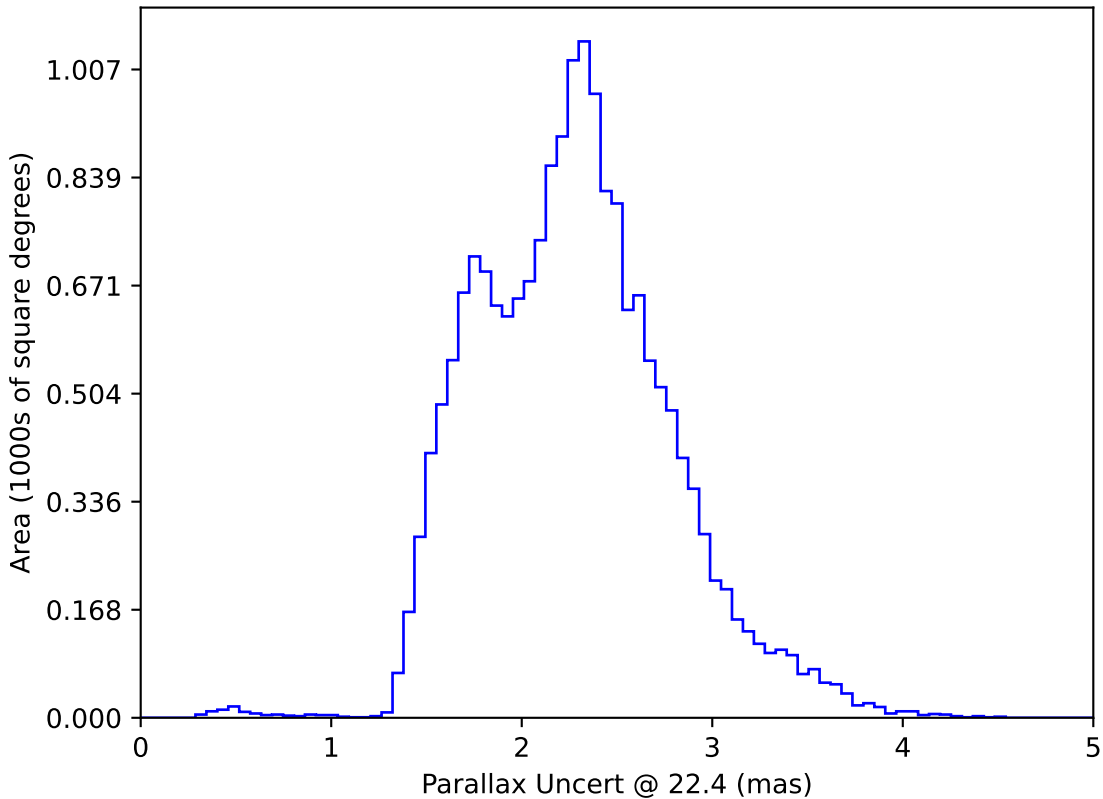
weather_cloudso36v3.4_10yrs WFD: Parallax Uncert @ 22.4
