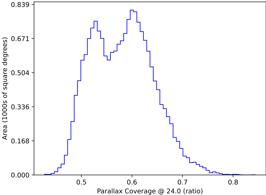
weather_cloudso36v3.4_10yrs WFD: Parallax Coverage @ 24.0
