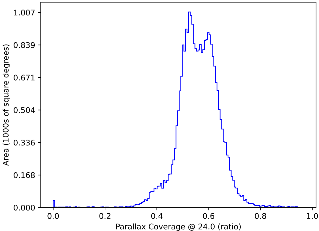
weather_cloudso36v3.4_10yrs All sky: Parallax Coverage @ 24.0
