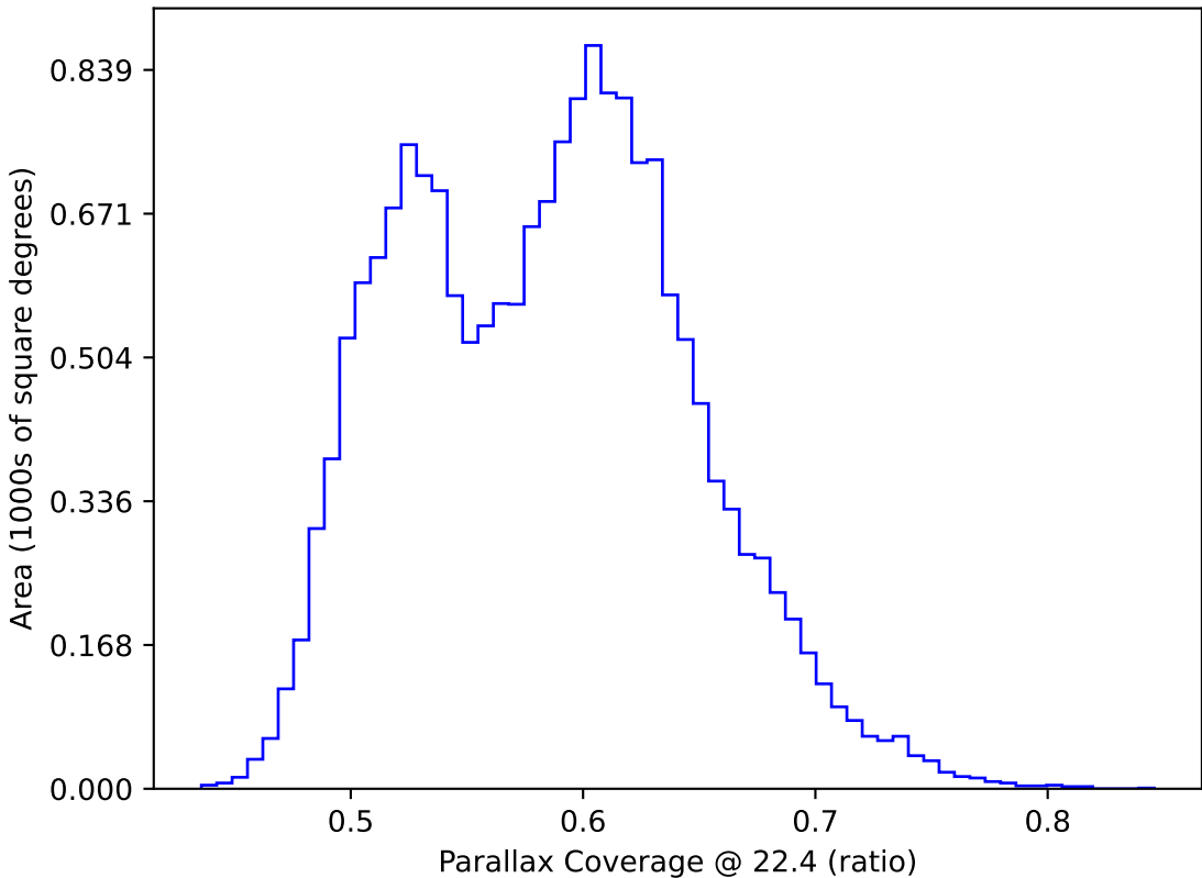
weather_cloudso36v3.4_10yrs WFD: Parallax Coverage @ 22.4
