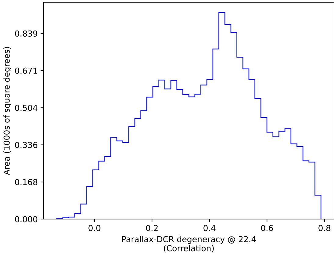
weather_cloudso36v3.4_10yrs WFD: Parallax-DCR degeneracy @ 22.4
