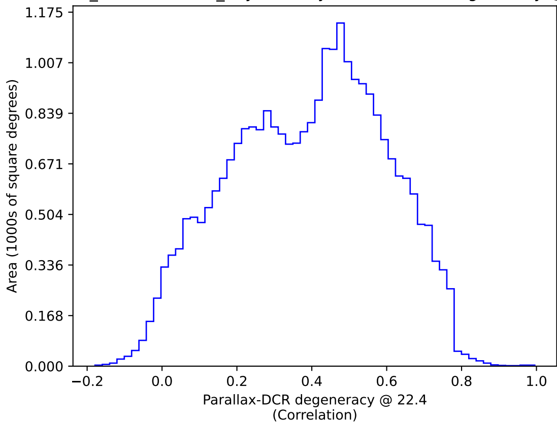
weather_cloudso36v3.4_10yrs All sky: Parallax-DCR degeneracy @ 22.4
