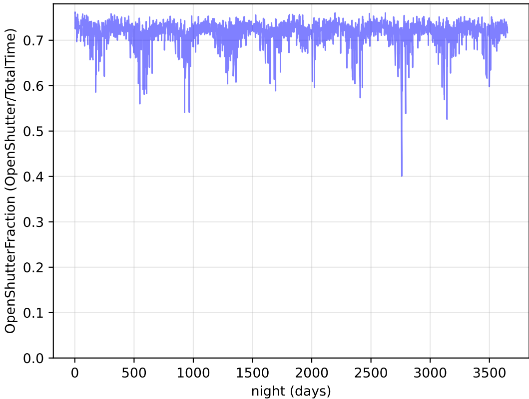
weather_cloudso36v3.4_10yrs Per night: OpenShutterFraction
