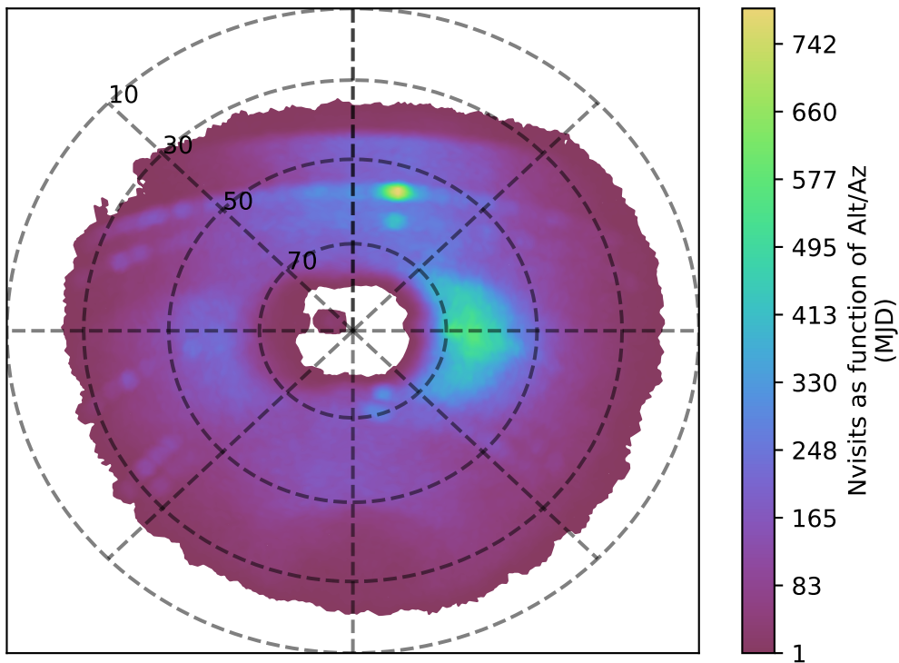
weather_cloudso36v3.4_10yrs u band: Nvisits as function of Alt/Az
