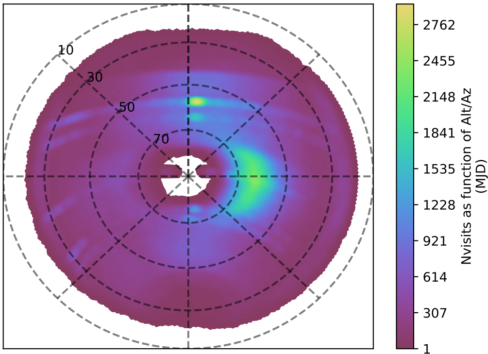
weather_cloudso36v3.4_10yrs i band: Nvisits as function of Alt/Az
