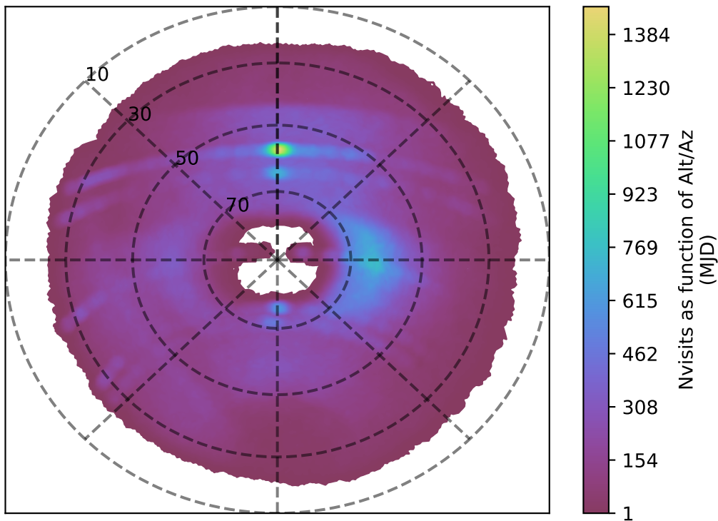
weather_cloudso36v3.4_10yrs g band: Nvisits as function of Alt/Az
