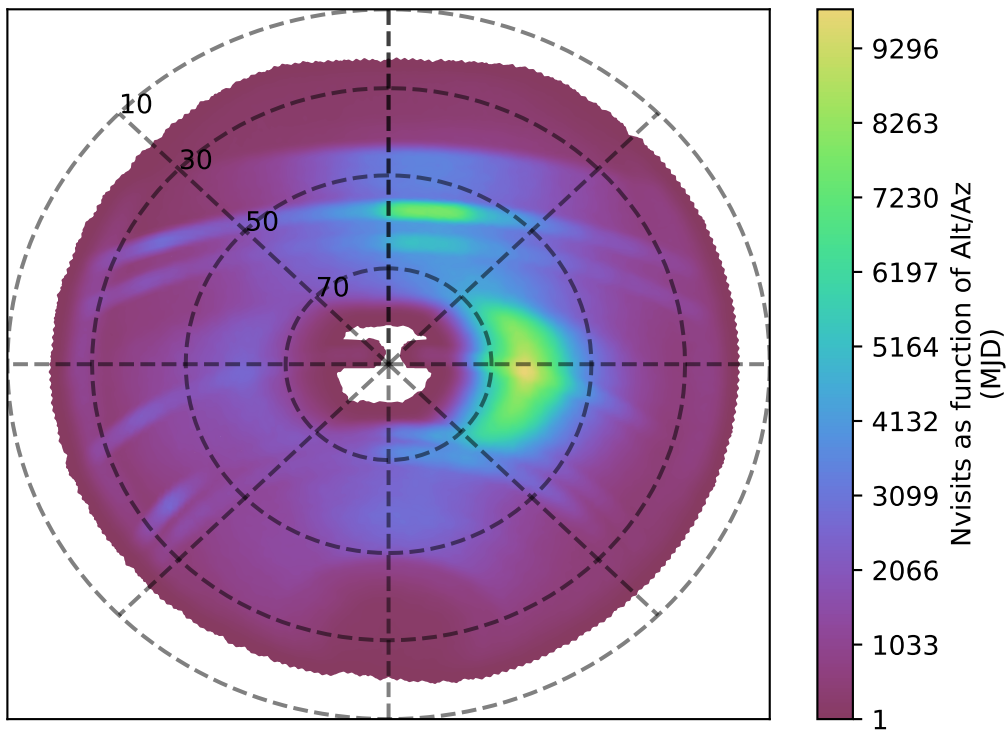
weather_cloudso36v3.4_10yrs all bands: Nvisits as function of Alt/Az
