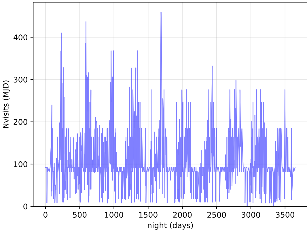
weather_cloudso36v3.4_10yrs DDF: Nvisits
