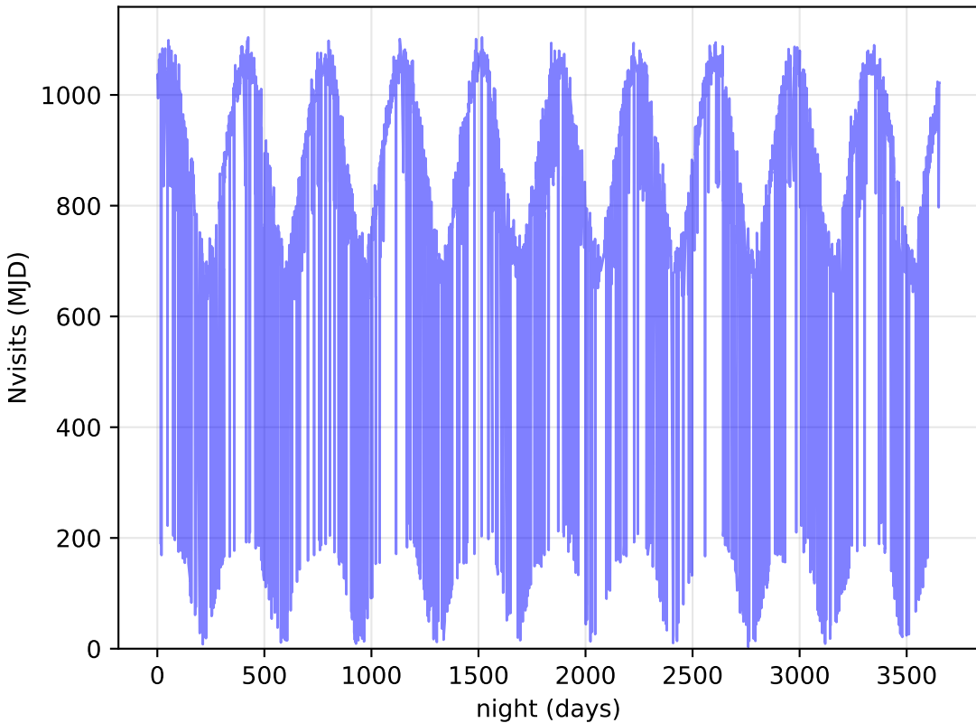
weather_cloudso36v3.4_10yrs All visits: Nvisits
