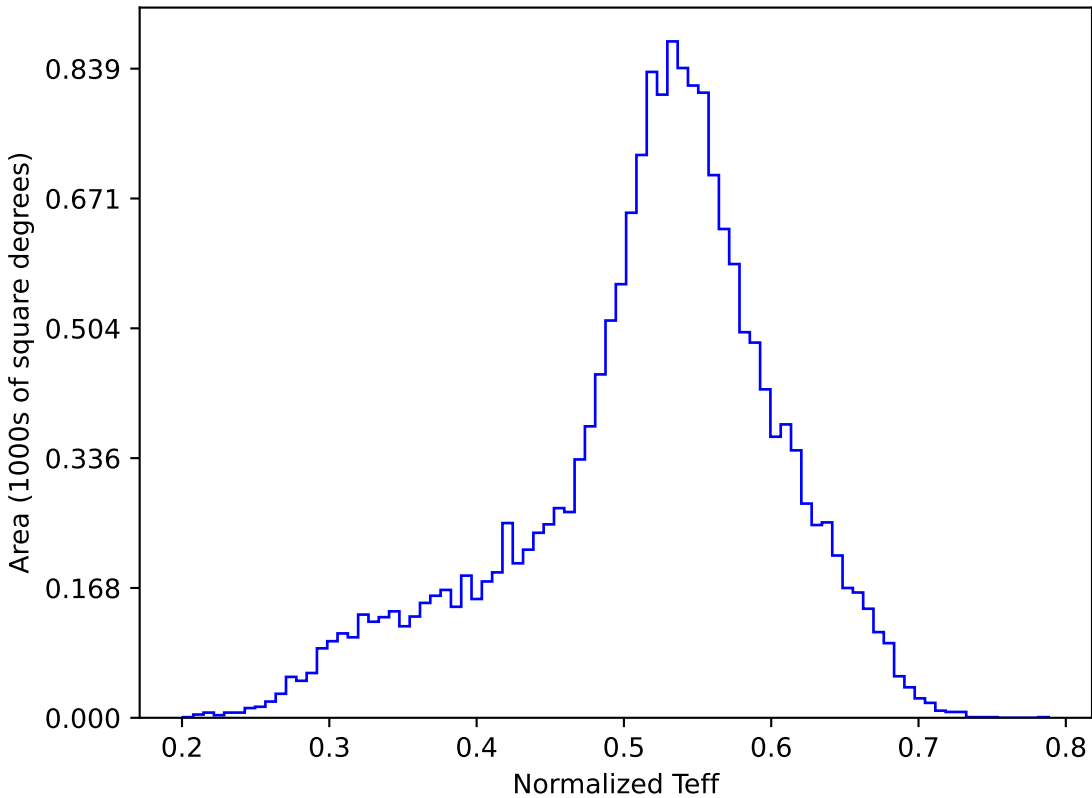
weather_cloudso36v3.4_10yrs WFD y band: Normalized Teff
