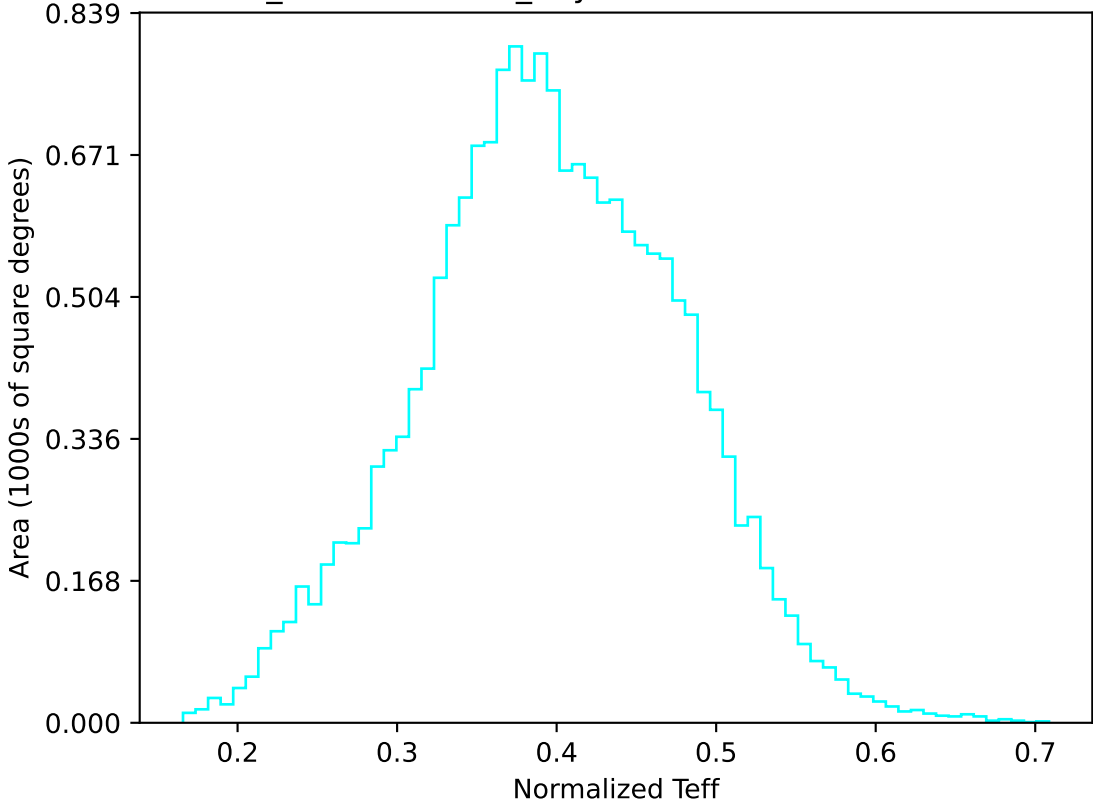
weather_cloudso36v3.4_10yrs WFD u band: Normalized Teff
