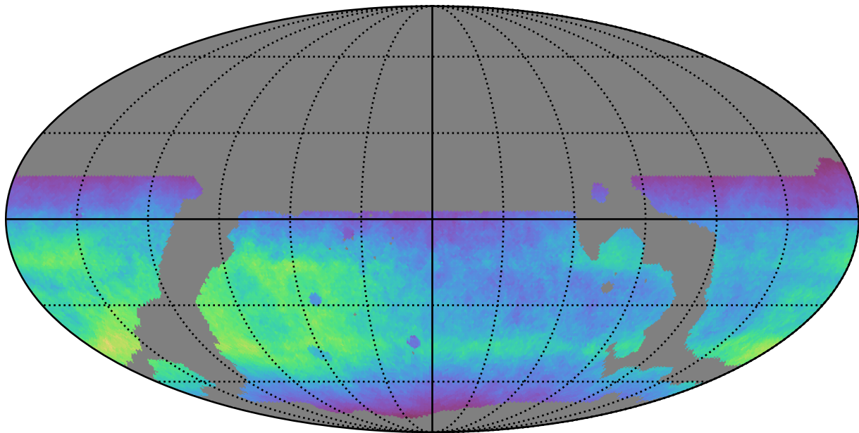
weather_cloudso36v3.4_10yrs WFD r band: Normalized Teff
