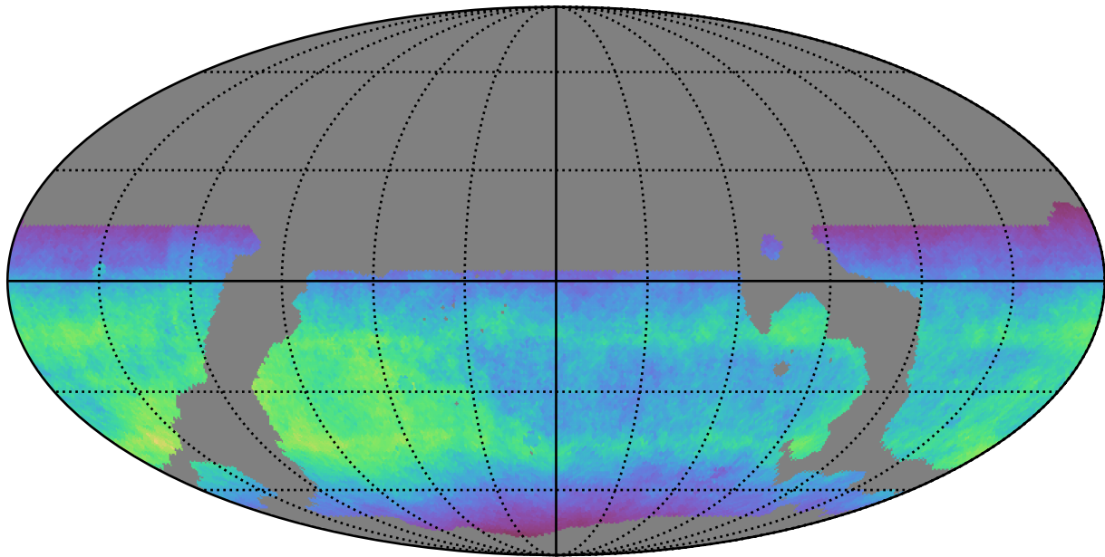
weather_cloudso36v3.4_10yrs WFD i band: Normalized Teff
