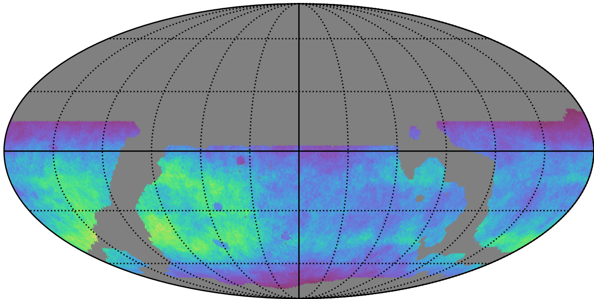
weather_cloudso36v3.4_10yrs WFD g band: Normalized Teff
