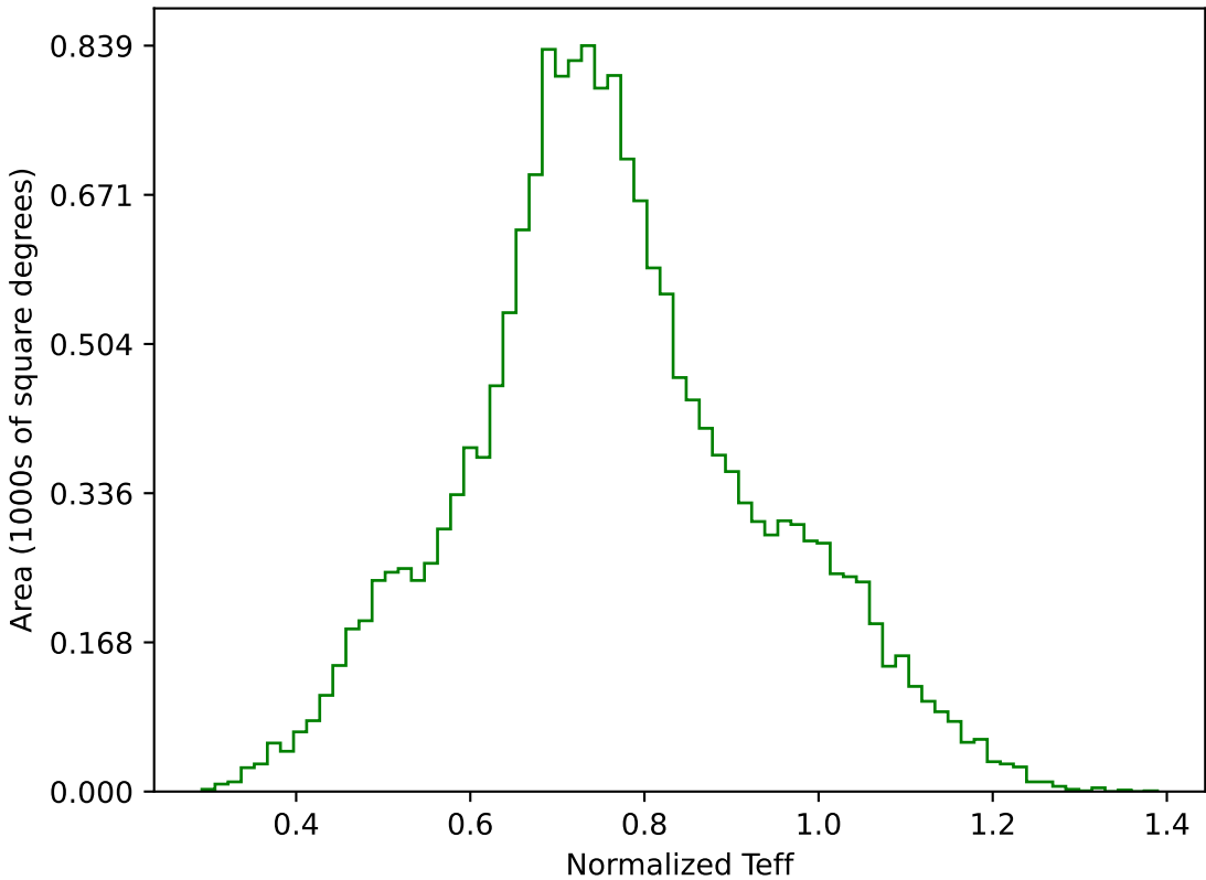
weather_cloudso36v3.4_10yrs WFD g band: Normalized Teff
