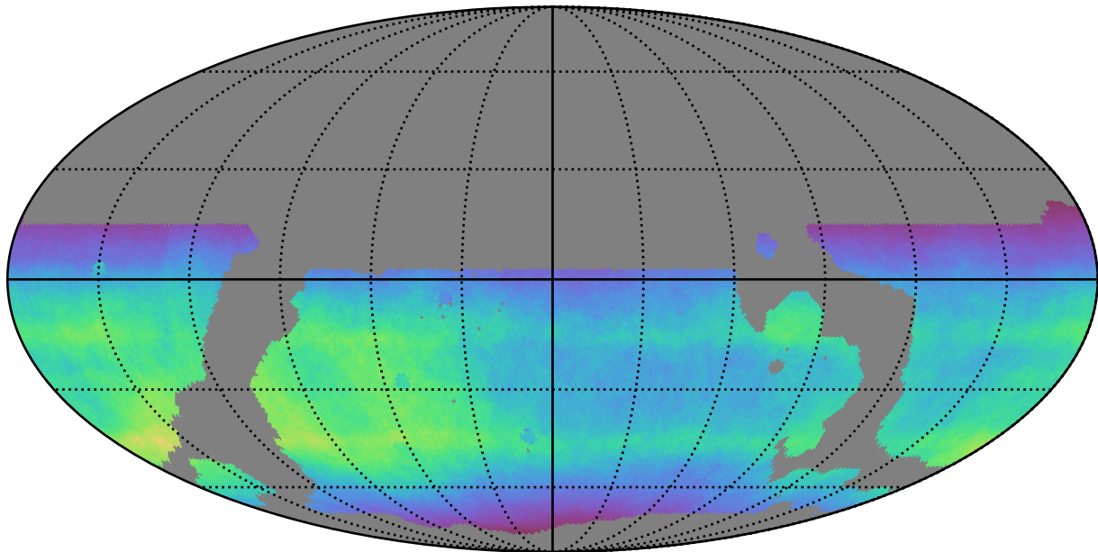
weather_cloudso36v3.4_10yrs WFD all bands: Normalized Teff
