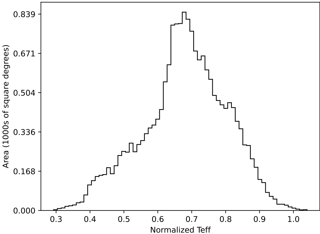
weather_cloudso36v3.4_10yrs WFD all bands: Normalized Teff
