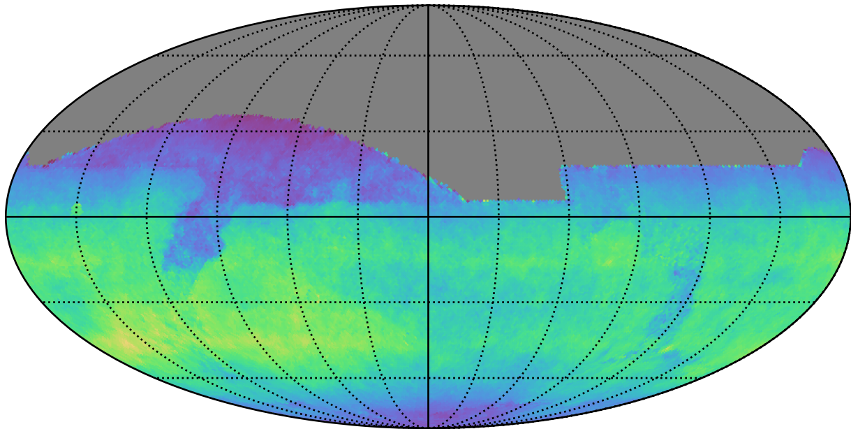
weather_cloudso36v3.4_10yrs All sky z band: Normalized Teff
