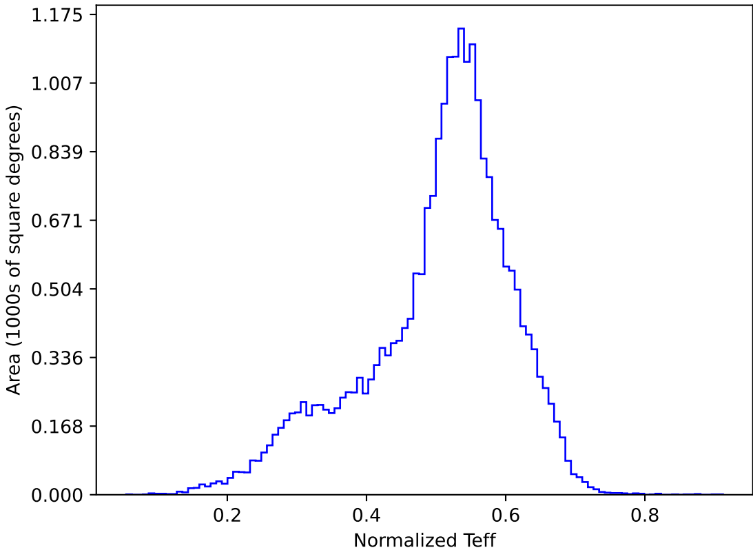
weather_cloudso36v3.4_10yrs All sky y band: Normalized Teff
