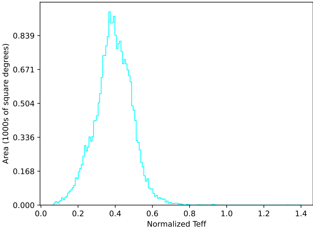
weather_cloudso36v3.4_10yrs All sky u band: Normalized Teff
