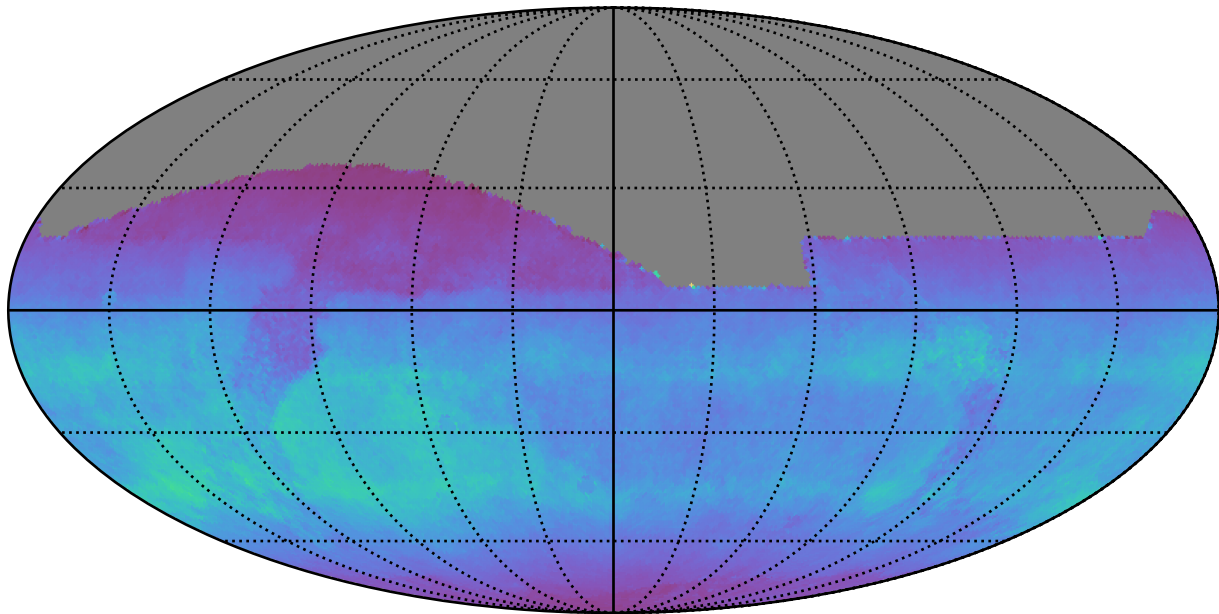
weather_cloudso36v3.4_10yrs All sky i band: Normalized Teff
