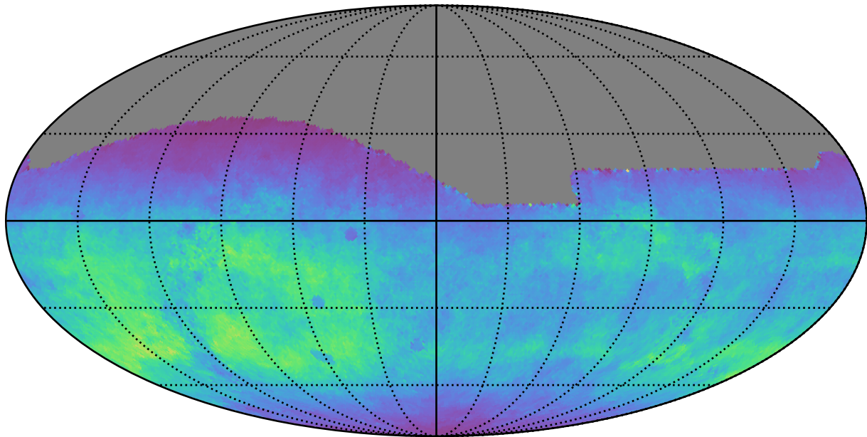
weather_cloudso36v3.4_10yrs All sky g band: Normalized Teff
