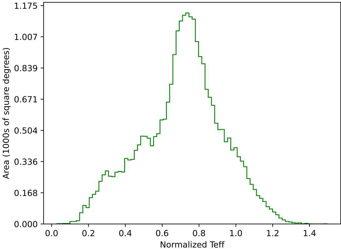
weather_cloudso36v3.4_10yrs All sky g band: Normalized Teff
