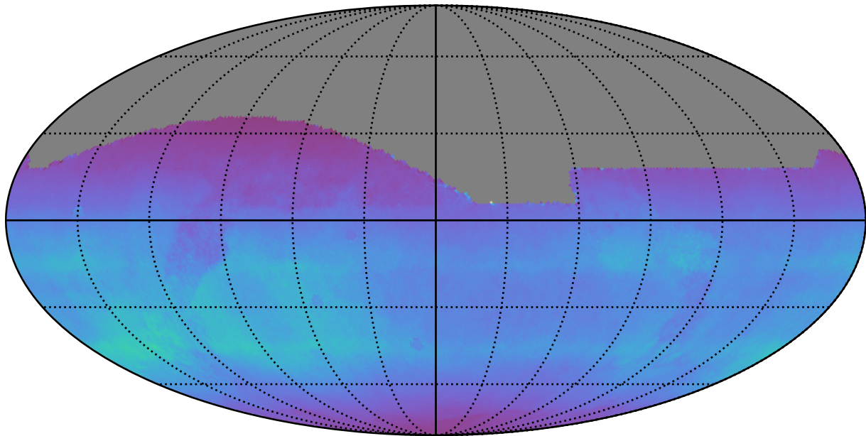
weather_cloudso36v3.4_10yrs All sky all bands: Normalized Teff
