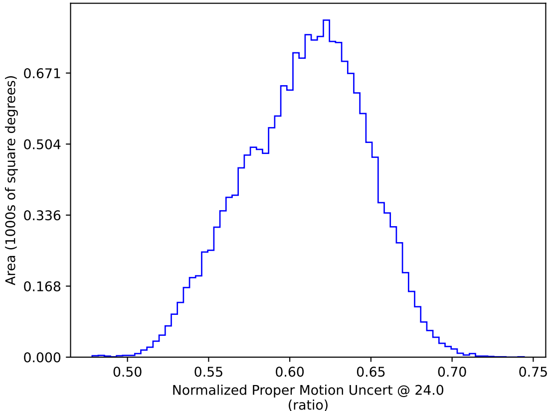
weather_cloudso36v3.4_10yrs WFD: Normalized Proper Motion Uncert @ 24.0
