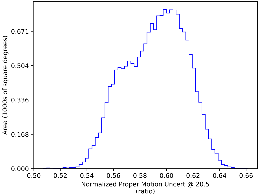
weather_cloudso36v3.4_10yrs WFD: Normalized Proper Motion Uncert @ 20.5
