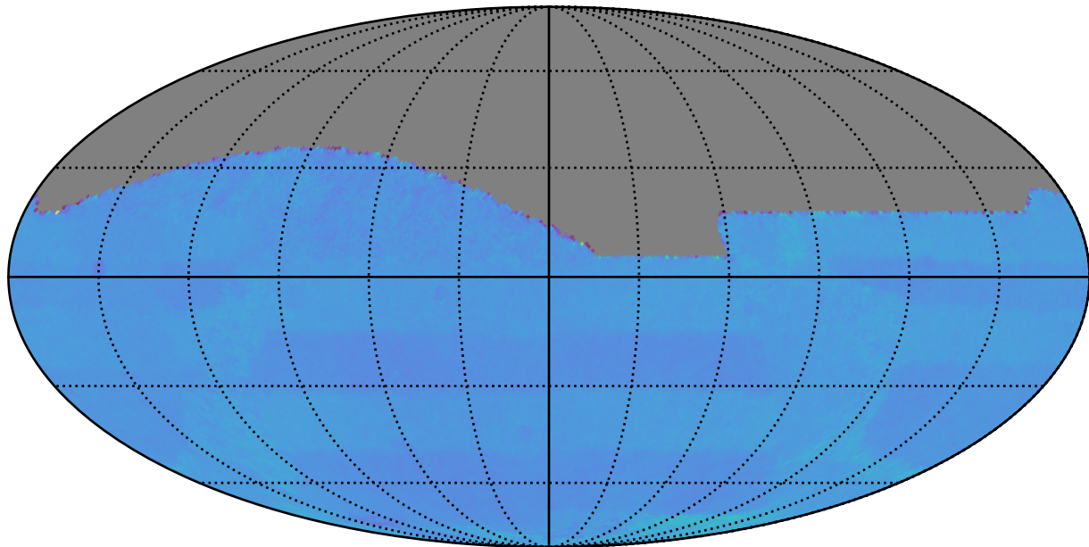
weather_cloudso36v3.4_10yrs All sky: Normalized Proper Motion Uncert @ 20.5
