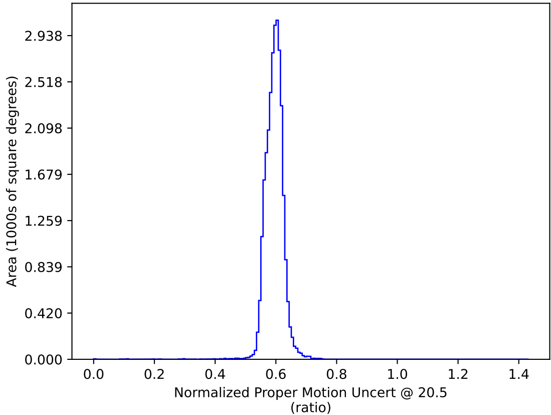
weather_cloudso36v3.4_10yrs All sky: Normalized Proper Motion Uncert @ 20.5
