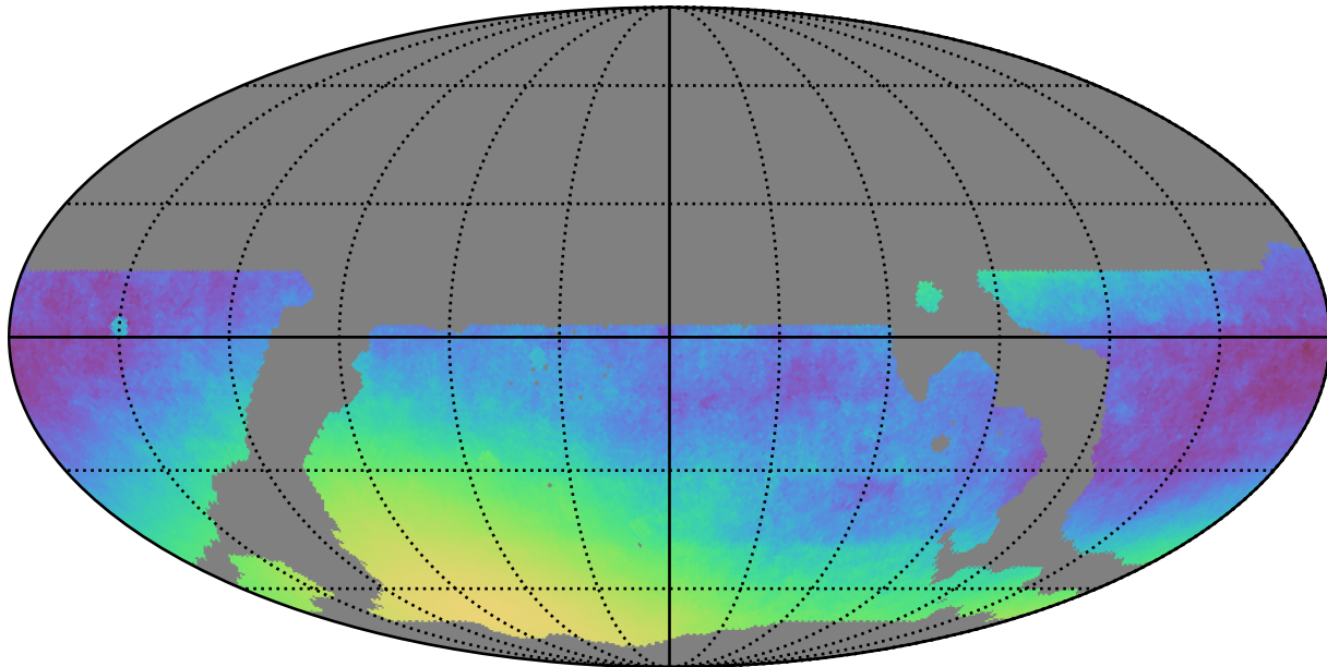
weather_cloudso36v3.4_10yrs WFD: Normalized Parallax Uncert @ 24.0
