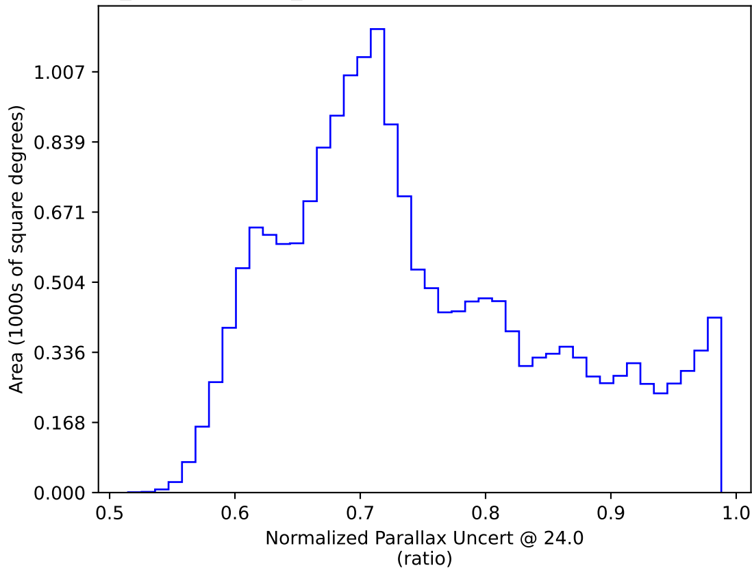
weather_cloudso36v3.4_10yrs WFD: Normalized Parallax Uncert @ 24.0
