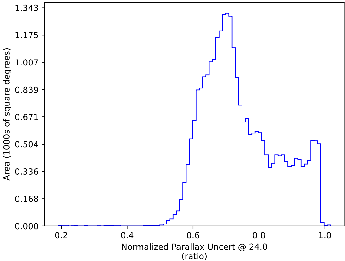
weather_cloudso36v3.4_10yrs All sky: Normalized Parallax Uncert @ 24.0
