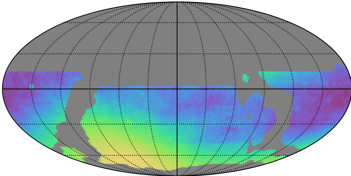
weather_cloudso36v3.4_10yrs WFD: Normalized Parallax Uncert @ 22.4
