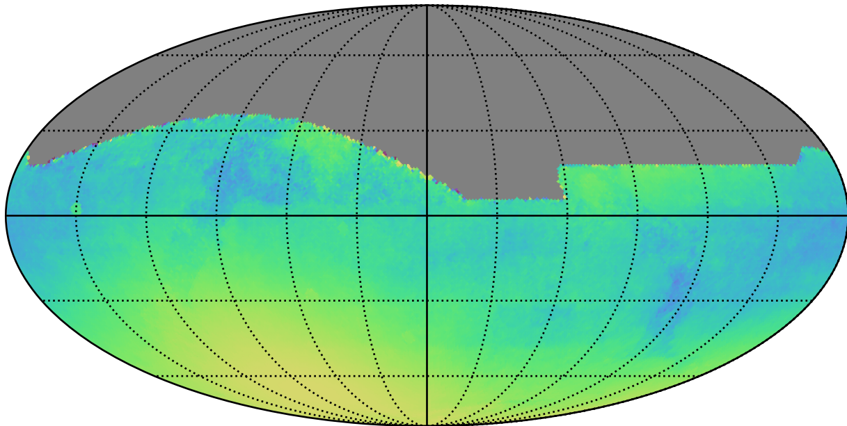
weather_cloudso36v3.4_10yrs All sky: Normalized Parallax Uncert @ 22.4
