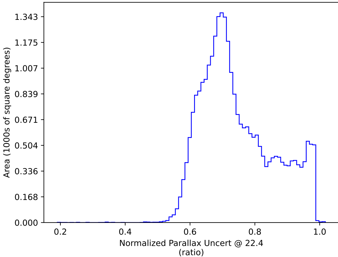
weather_cloudso36v3.4_10yrs All sky: Normalized Parallax Uncert @ 22.4
