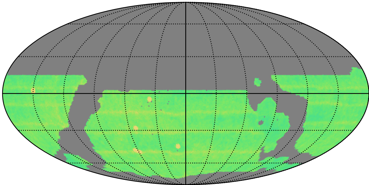
weather_cloudso36v3.4_10yrs WFD all bands: N Unique Nights
