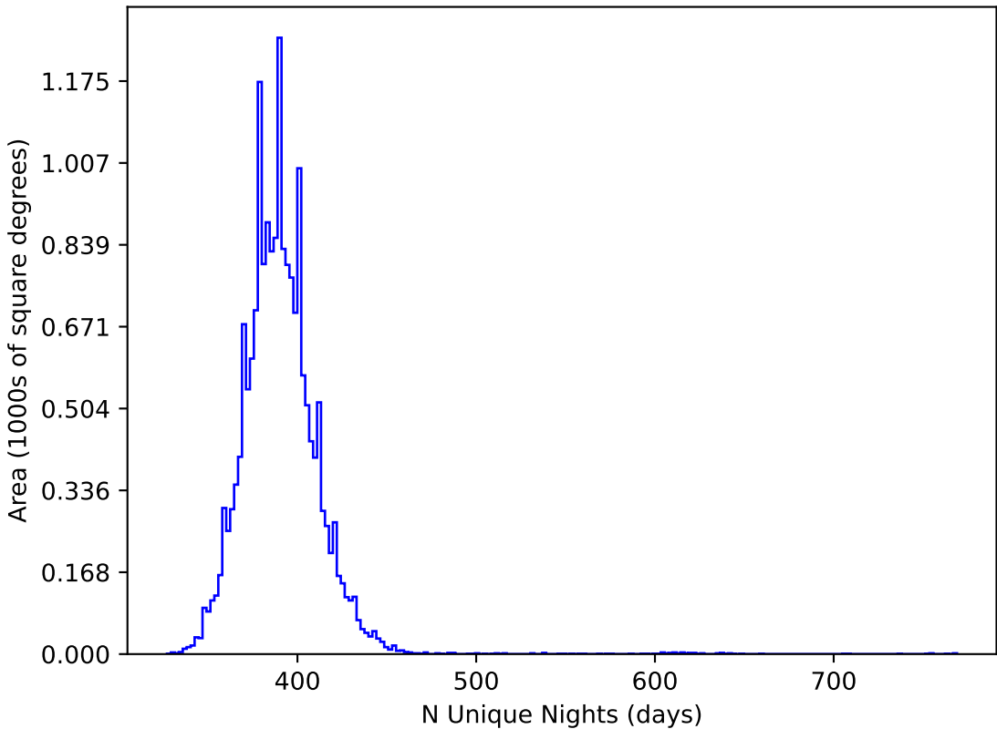
weather_cloudso36v3.4_10yrs WFD all bands: N Unique Nights
