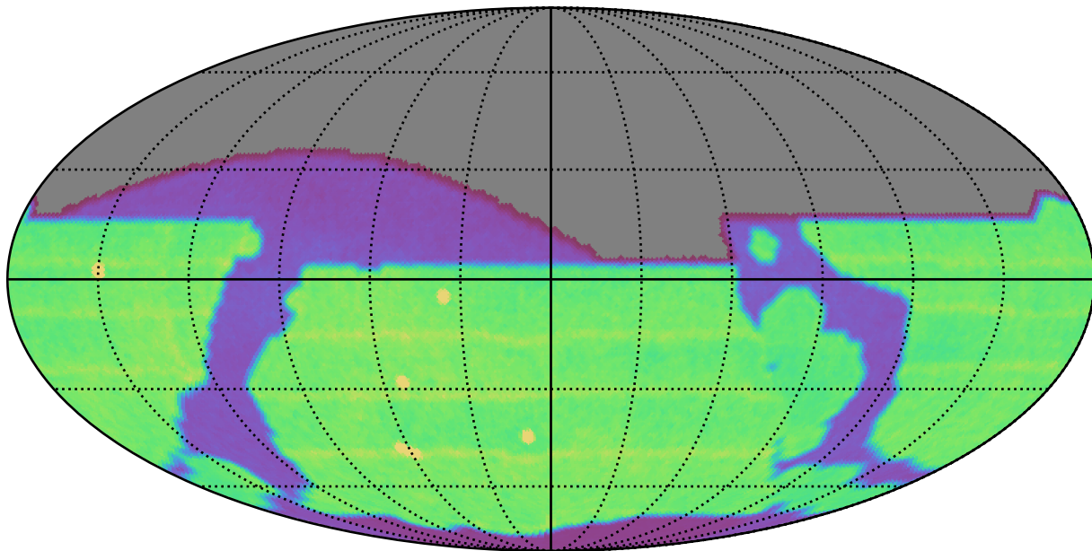
weather_cloudso36v3.4_10yrs All sky all bands: N Unique Nights
