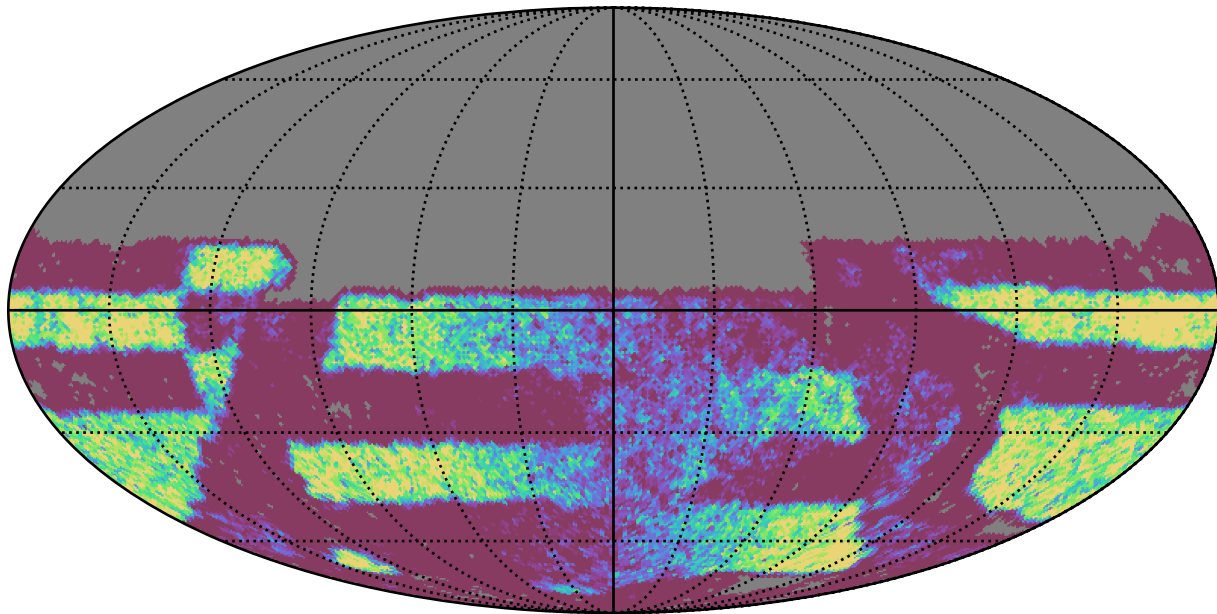
weather_cloudso36v3.4_10yrs Yr 3-4 y band: NVisits
