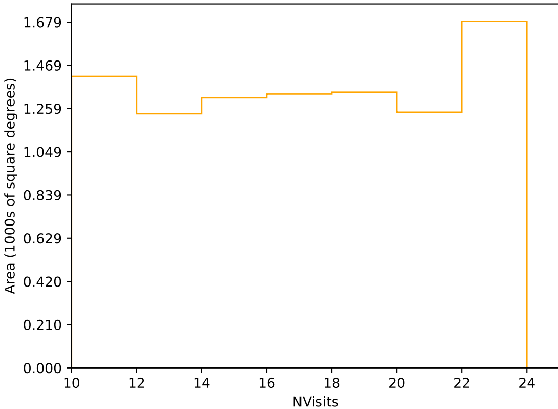
weather_cloudso36v3.4_10yrs Yr 3-4 r band: NVisits
