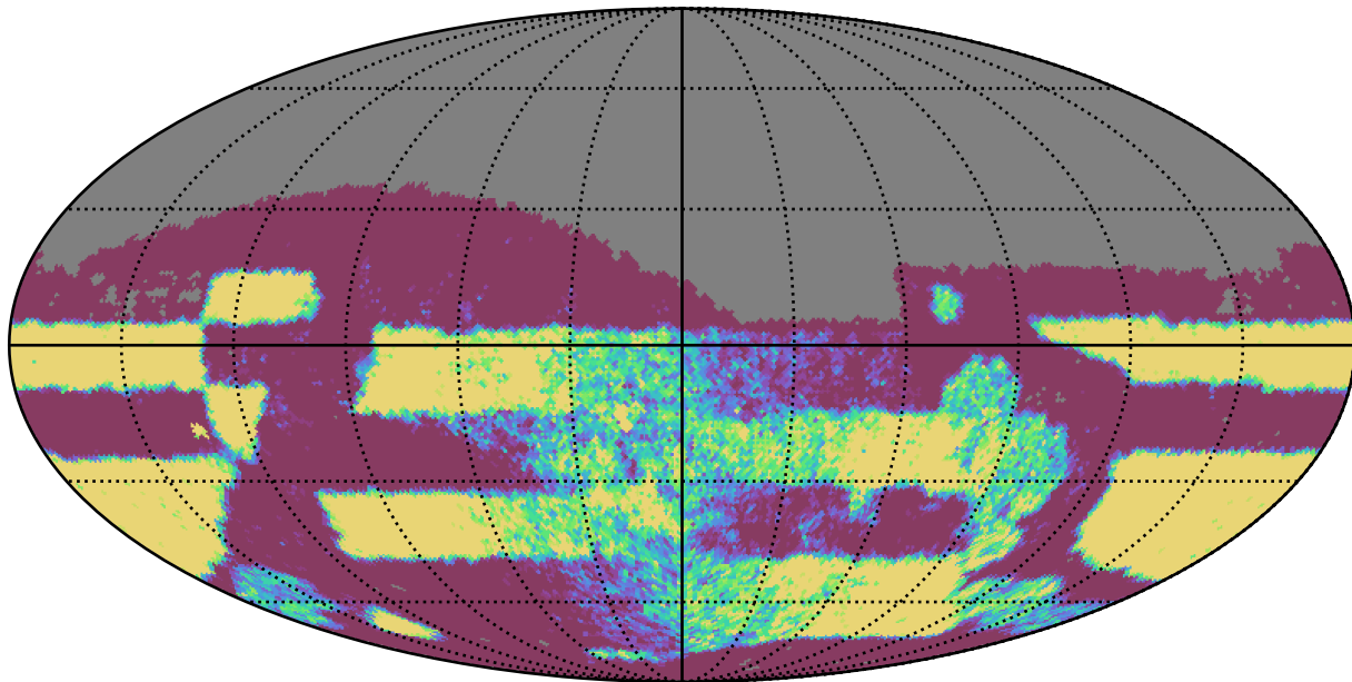
weather_cloudso36v3.4_10yrs Yr 3-4 i band: NVisits
