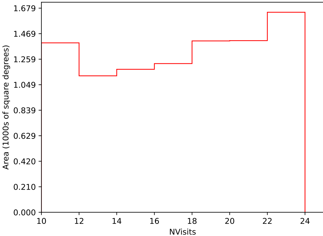
weather_cloudso36v3.4_10yrs Yr 3-4 i band: NVisits
