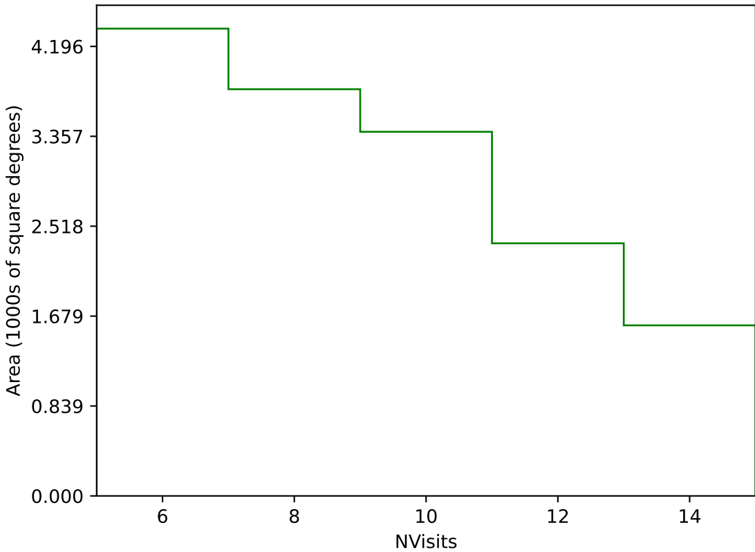
weather_cloudso36v3.4_10yrs Yr 3-4 g band: NVisits
