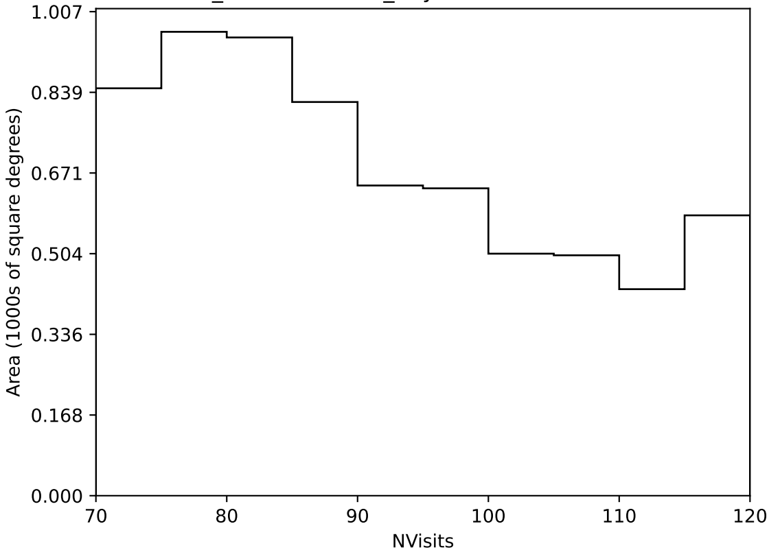
weather_cloudso36v3.4_10yrs Yr 3-4 all bands: NVisits
