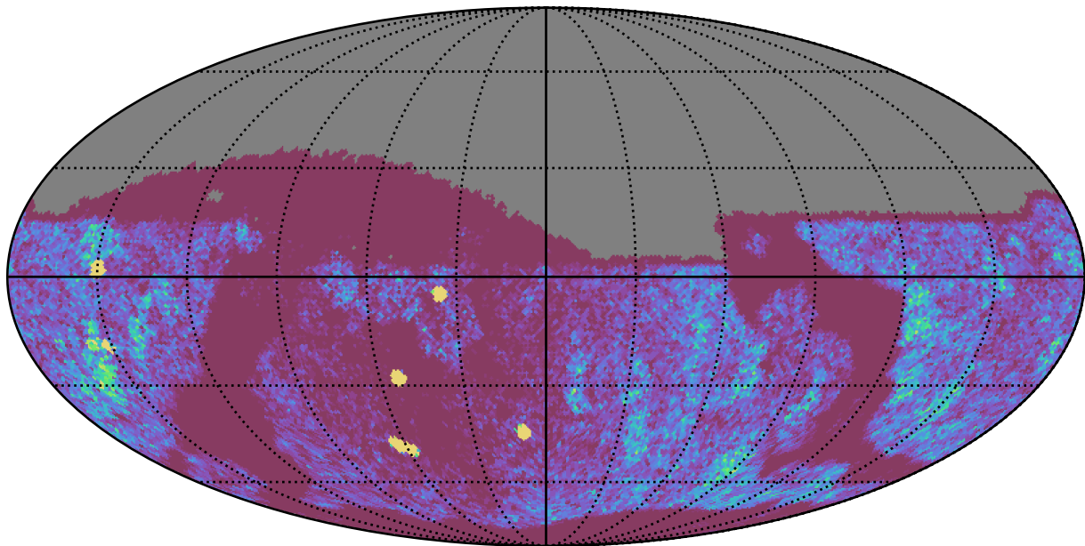
weather_cloudso36v3.4_10yrs Yr 1 z band: NVisits
