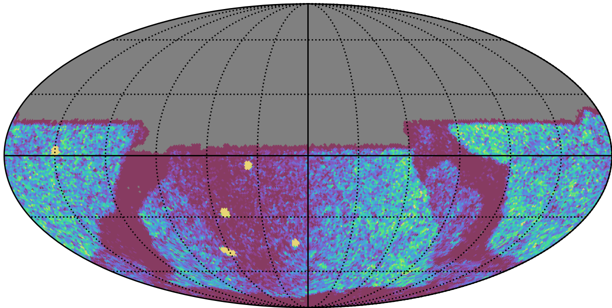
weather_cloudso36v3.4_10yrs Yr 1 y band: NVisits
